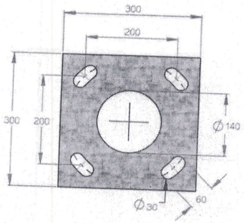
BASE PLATE DETAIL SCALE 1 : 8
